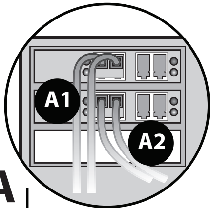
Sun StorEdge 5310 NAS connected to a 5300 RAID EU and a single EU-F Expansion Enclosure
